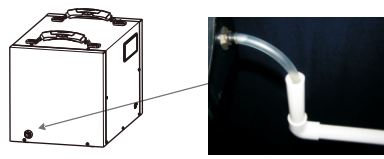
Drain Tube – 12 inches Long, 19 mm OD.
