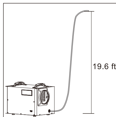
Pump Drain
